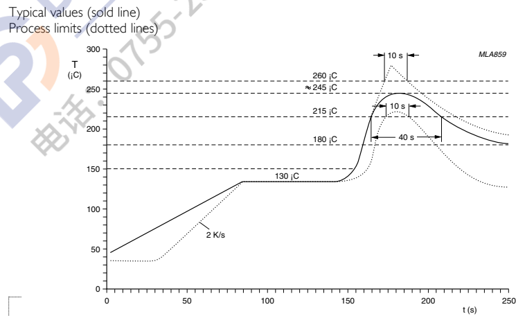
Fig. 7 Recommended reflow soldering profile
