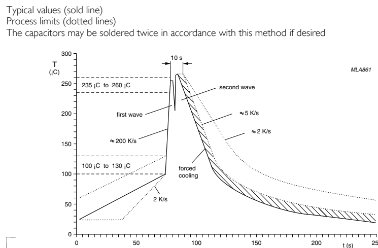
Fig. 8 Recommended wave soldering profile
